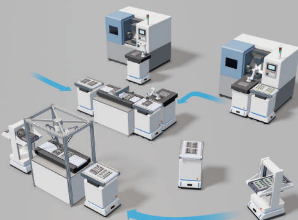
Work Transportation Robots Between Each Process
